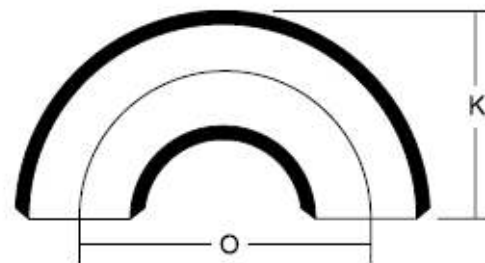
180° Return/Long Radius
